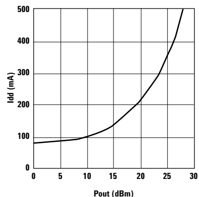
Figure 13. Idd vs. Pout.
