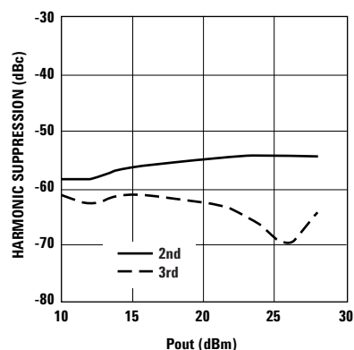
Figure 16. 2nd/3rd Harmonics vs. Pout.
